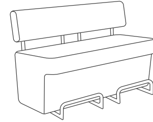
Work Height Double W 54.5 x D 29.0 x H 39.5 SH 24.0 x SD 20.0 Weight Approx 125 lbs
