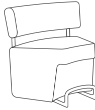
Work Height Inside 45 W 38.0 x D 29.0 x H 39.5 SH 24.0 x SD 20.0 Weight Approx 75 lbs
